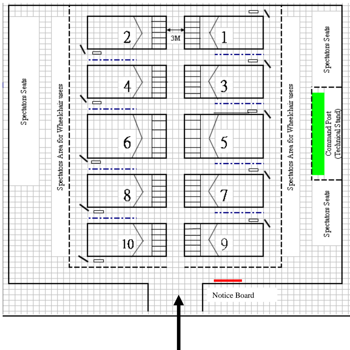
Floor Plan of Competition Area
